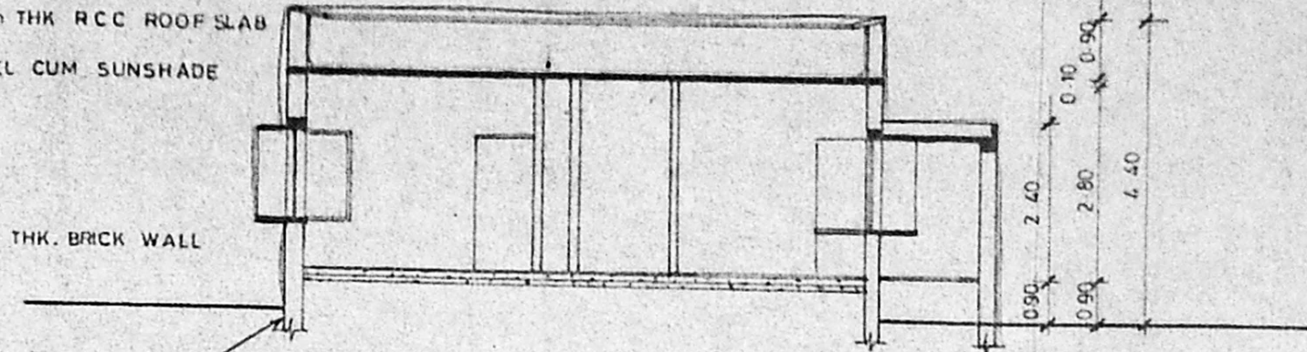
SECTION B-B
